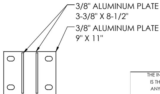
STD. MOUNTING BRACKET
